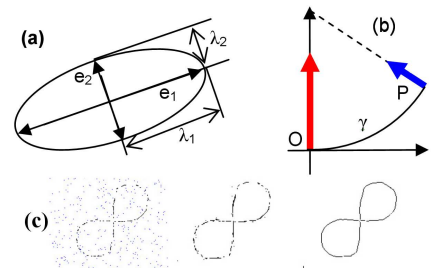
Figure 5: Tensor Voting: (a) tensor ellipse, (b) 2D stick kernel, (c) Tensor voting example: left image shows the sparse input tokens without orientation, middle image is the tokens oriented by tensor voting but still sparse, the right image is the resulting extracted dense curve.
